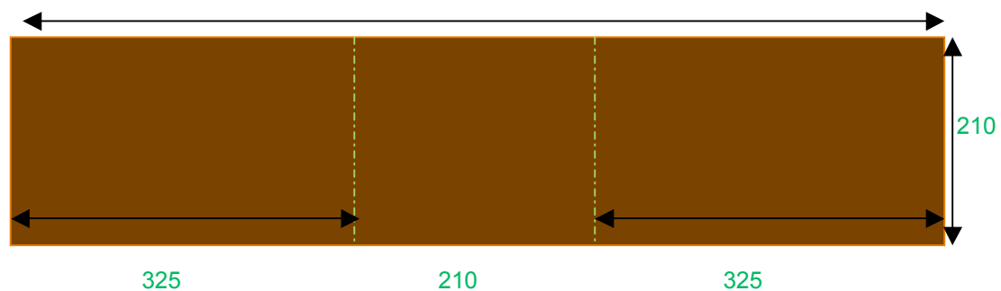
Figure 4.2 Fold the sheet metal to make the sides and bottom of the combustion chamber
